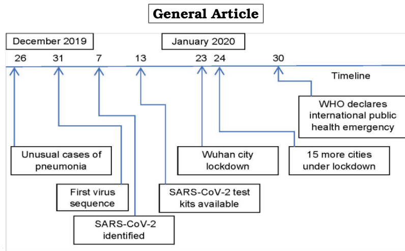
Figure 7: Wuhan Covid-19 outbreak timeline
