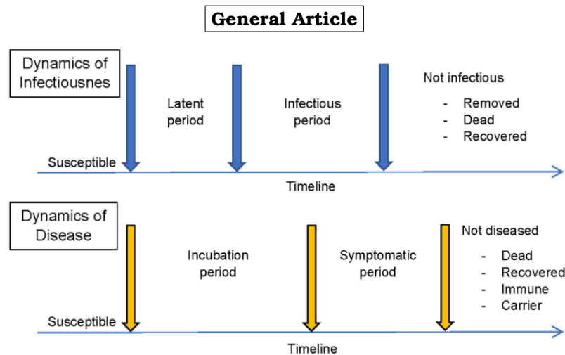
Figure 5: Dynamics of infection and disease (modified from [1])
